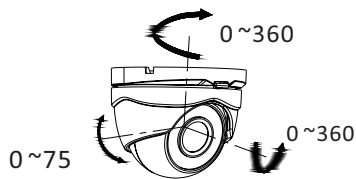
Figure 2-4 3-axis Adjustment
